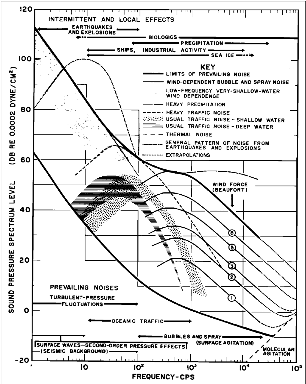
Figure 1-7: Generalised ambient noise spectra attributable to various noise sources (Wenz, 1962).
